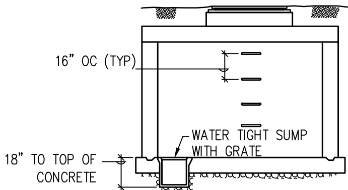
SECTION B
