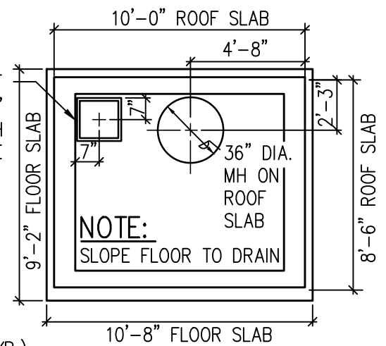
FLOOR & ROOF PLAN
