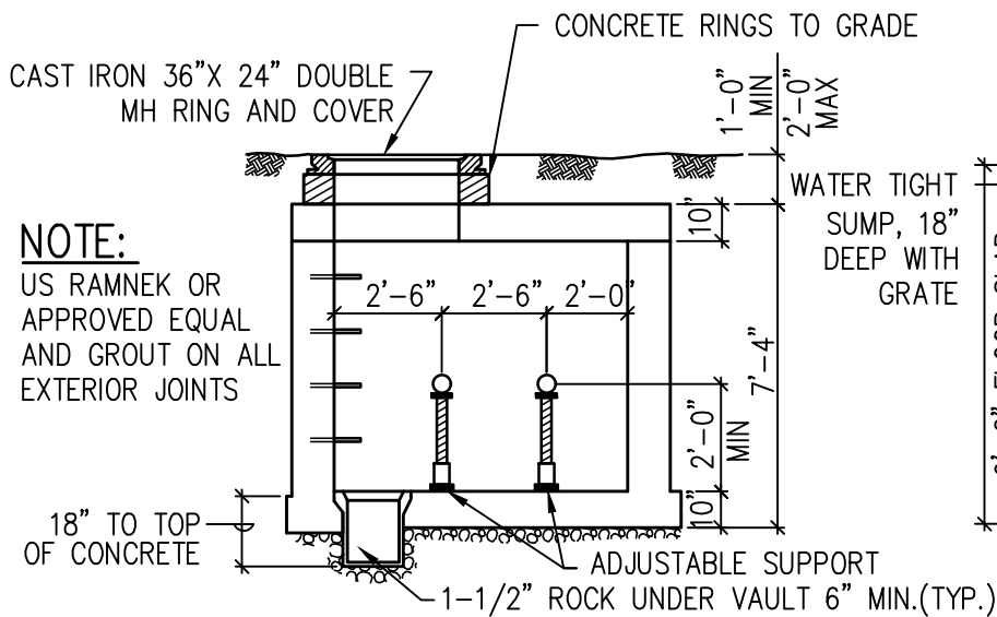
SECTION A
