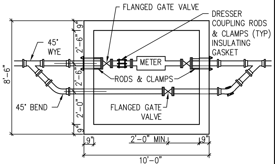
VAULT PLAN
