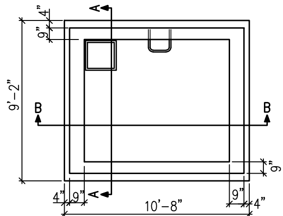
VAULT PLAN
