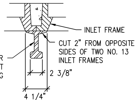
RAIL DETAIL
