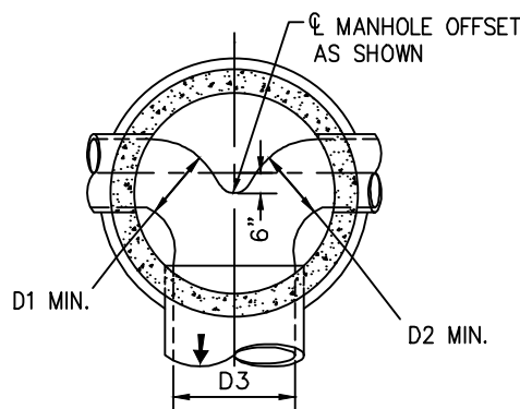
OPPOSED LATERALS
