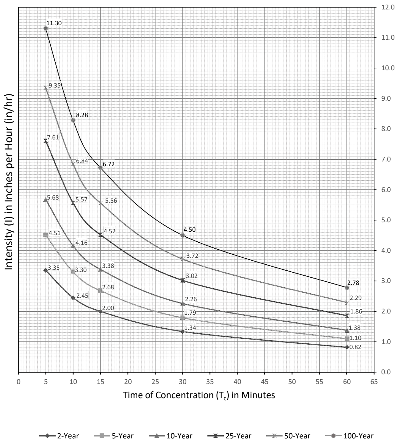
Figure 600- 1: Town of Berthoud – Intensity-Duration-Frequency Curves
